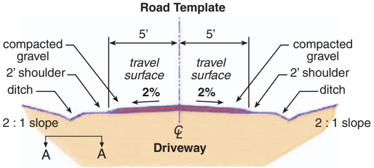
Road Grade Profile – Scale: 1"=50' Horiz. 1"=10' Vert.
