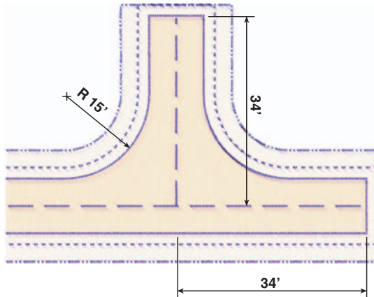
Hammerhead Turnaround Detail
